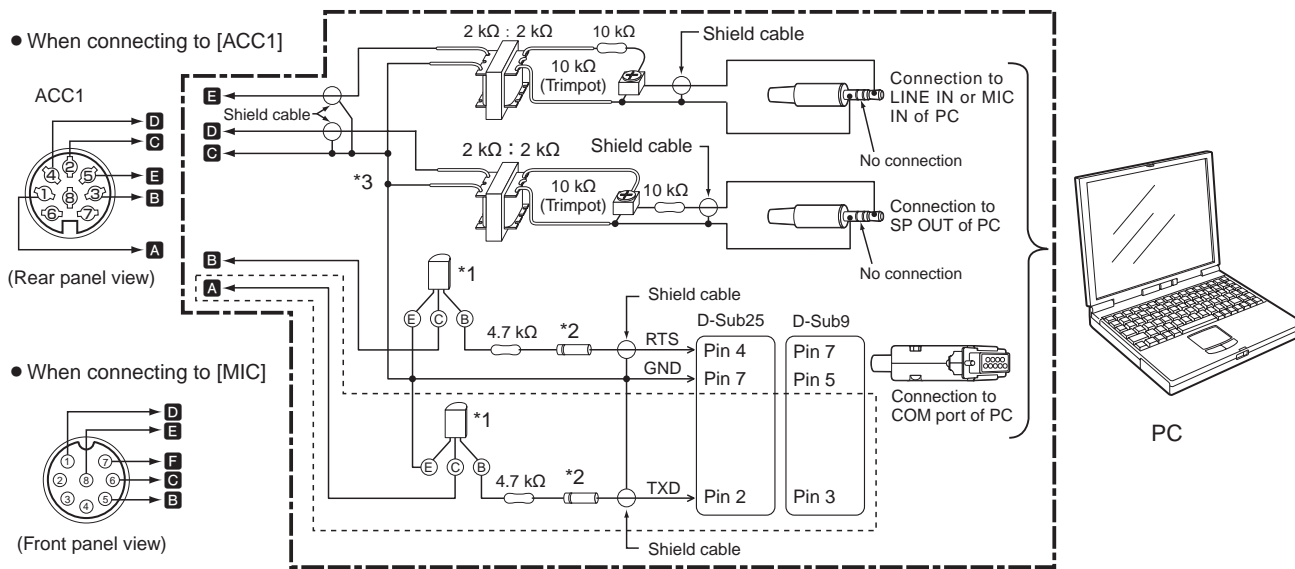
Example interface circuit for digital modes (Not provided by Icom)
