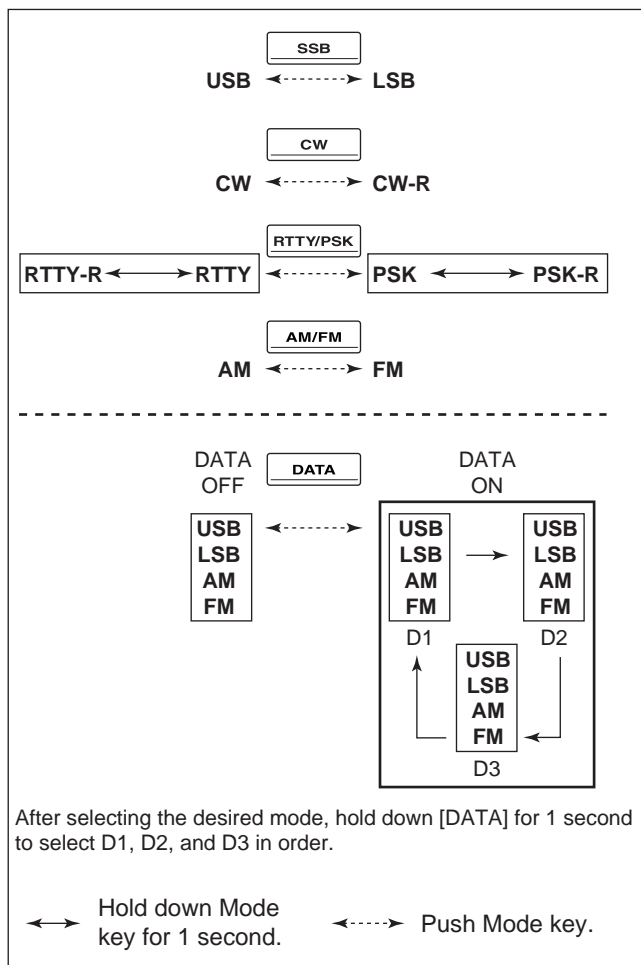
Mode keys
